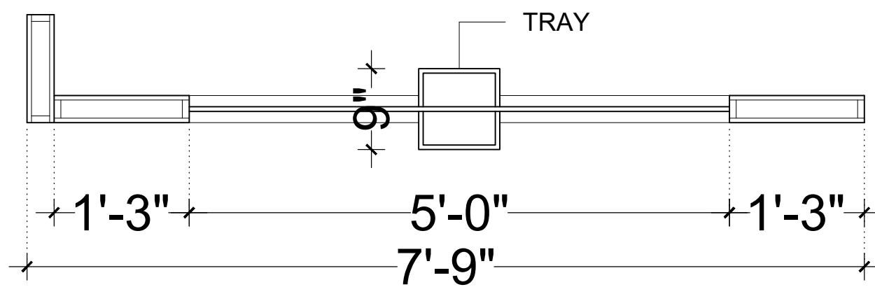
PLAN (PT4)
