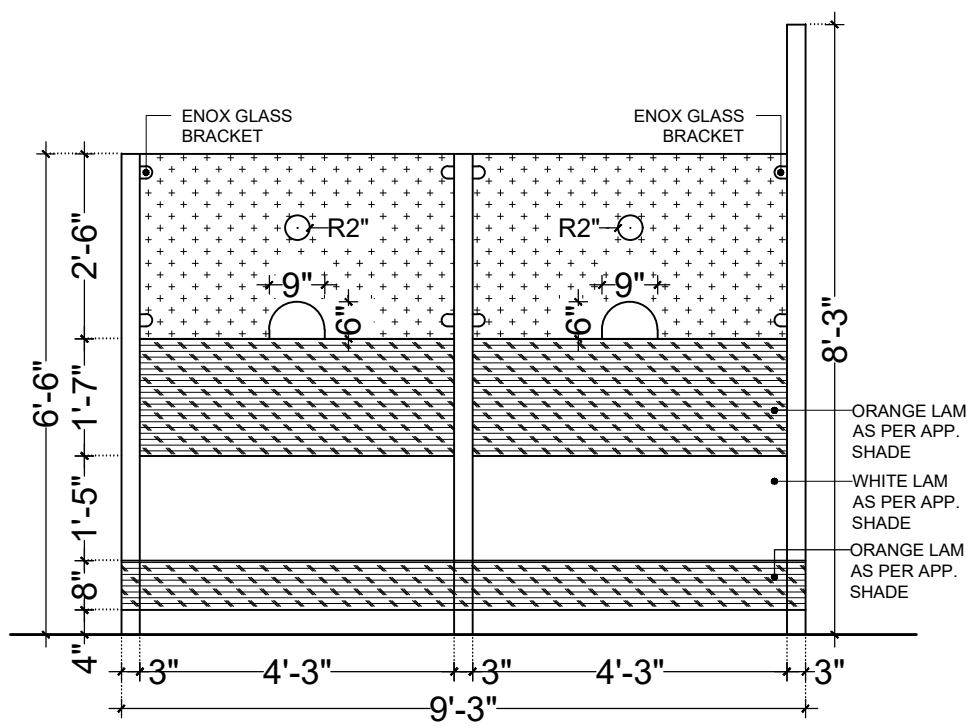
ELEVATION (FRONT)
