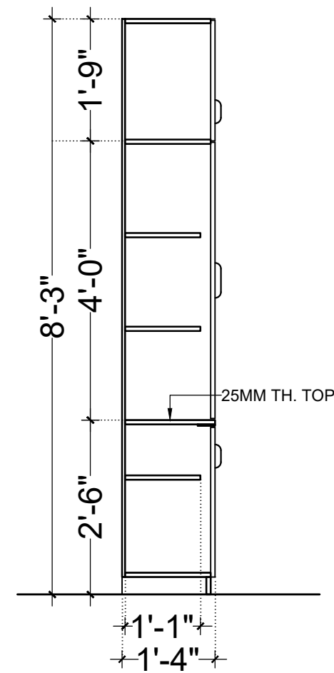
SECTION AA (CB1)
