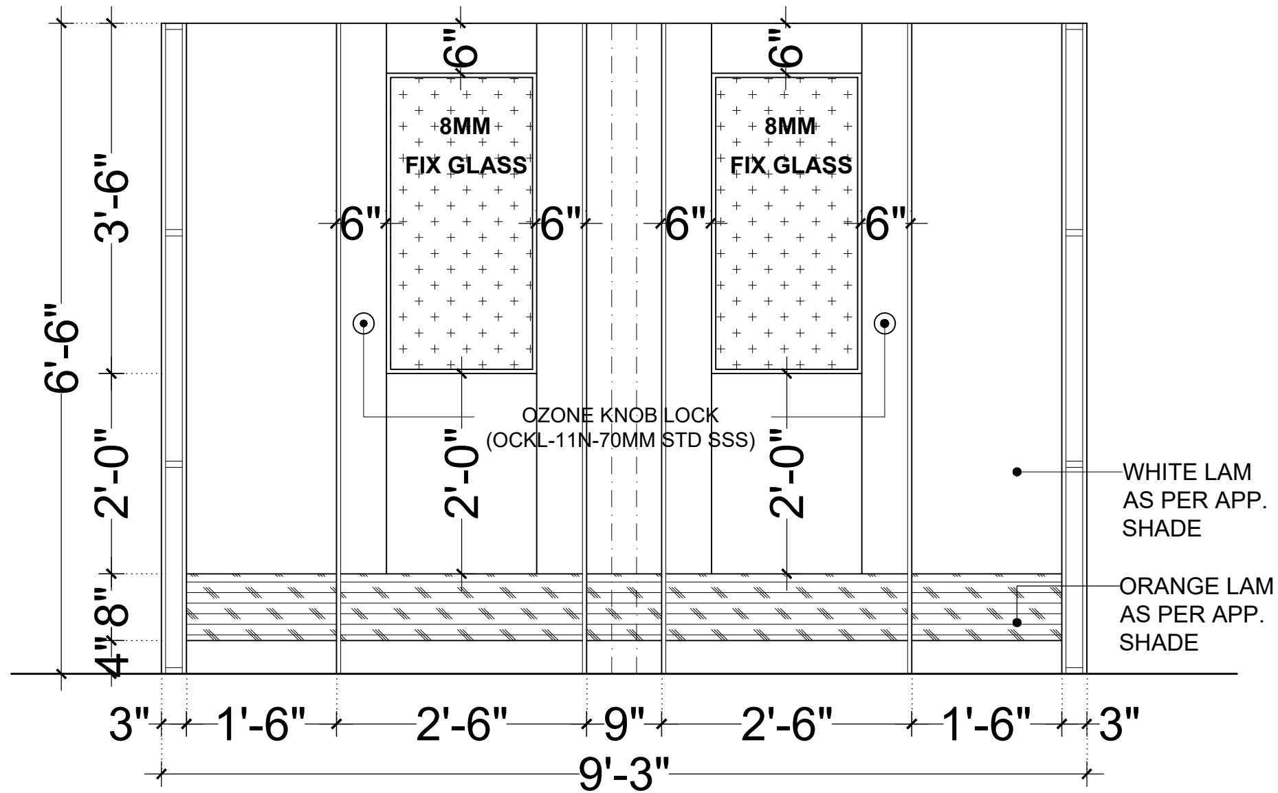
ELEVATION (PT6)
