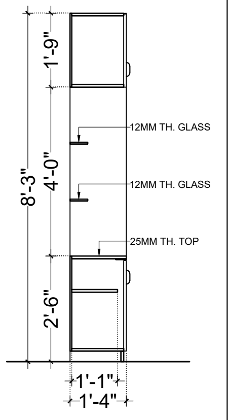
SECTION CC (CB3)
