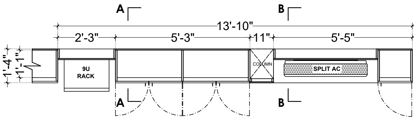
PLAN (CB2) (LVL + 7'-0")
