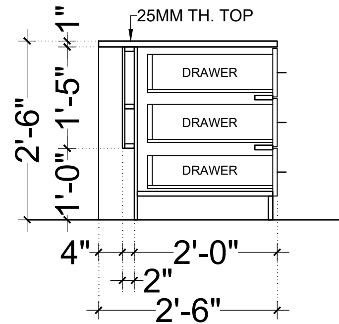
SECTION AA (OT3)
