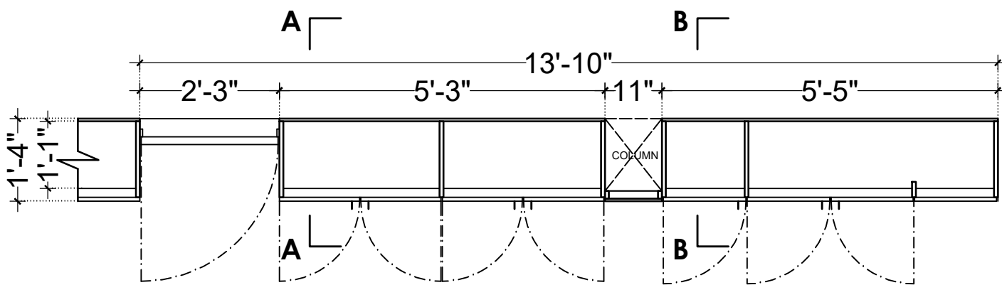
PLAN (CB2) (LVL + 2'-0")
