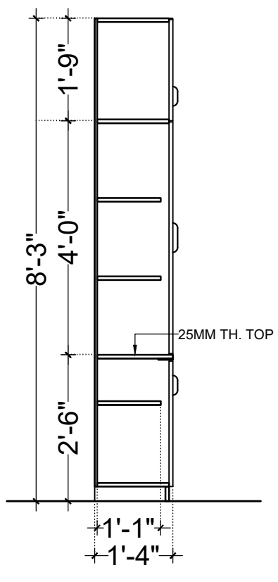
SECTION AA (CB3)
