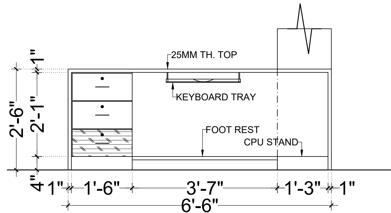
ELEVATION (INSIDE) (MT1)
