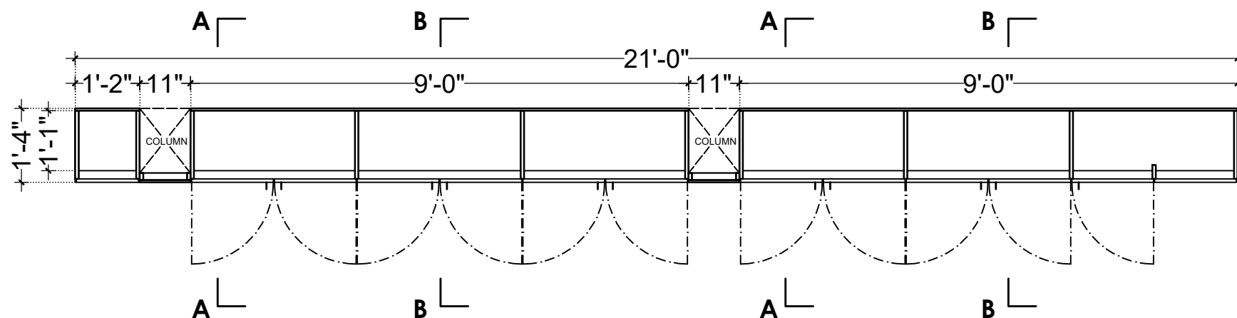
PLAN (CB4) (LVL + 2'-0")
