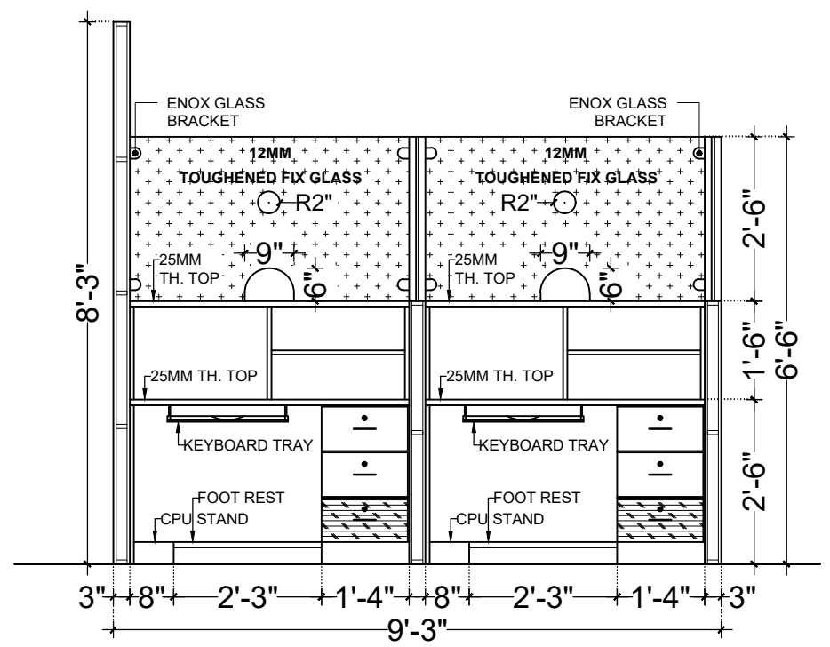
ELEVATION (INSIDE)
