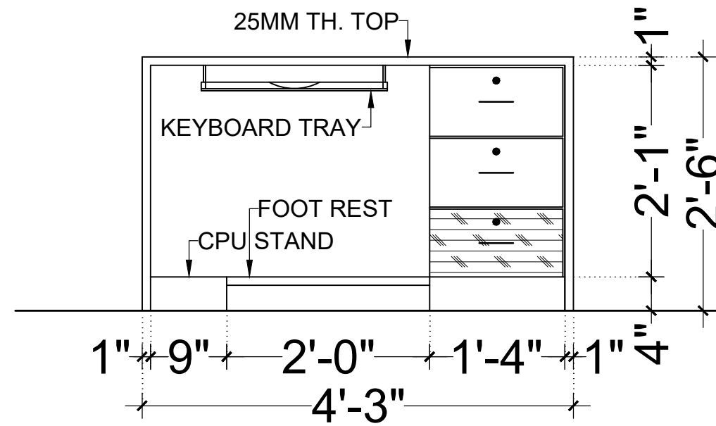
ELEVATION (INSIDE) (OT2)
