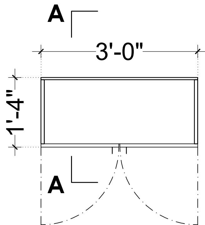
PLAN (LVL + 1'-6") (SC1)
