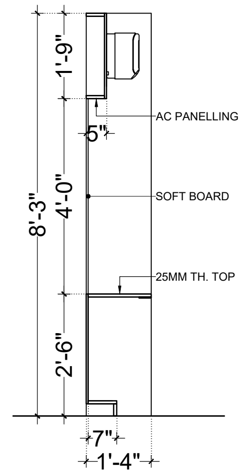
SECTION BB (CB5)
