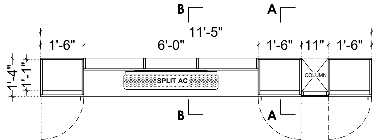
PLAN (CB1) (LVL + 7'-0")
