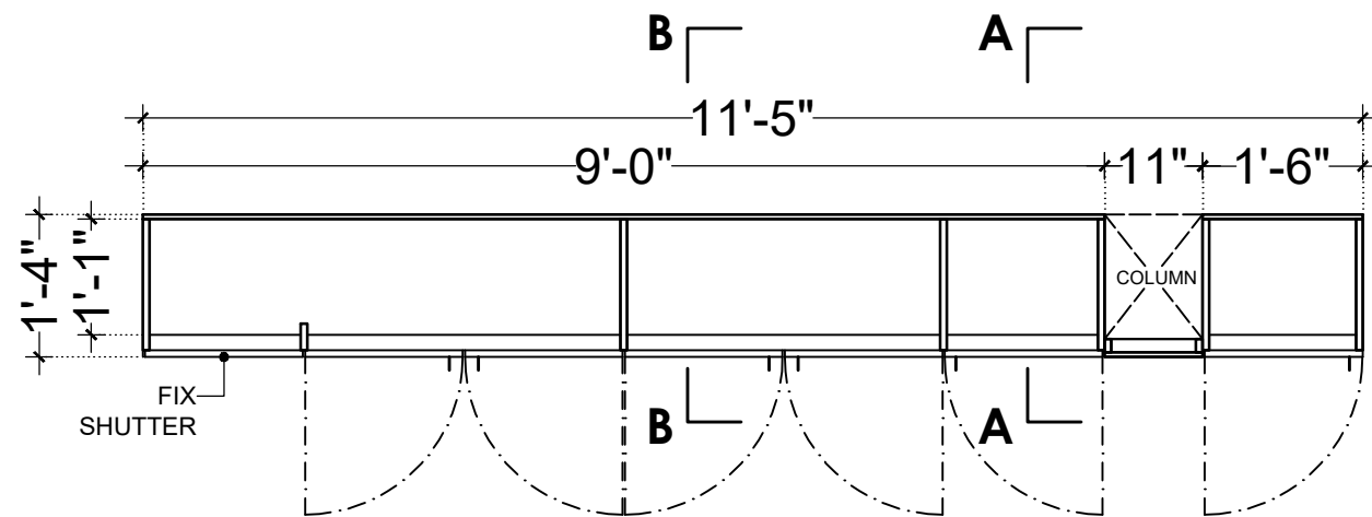
PLAN (CB1) (LVL + 2'-0")
