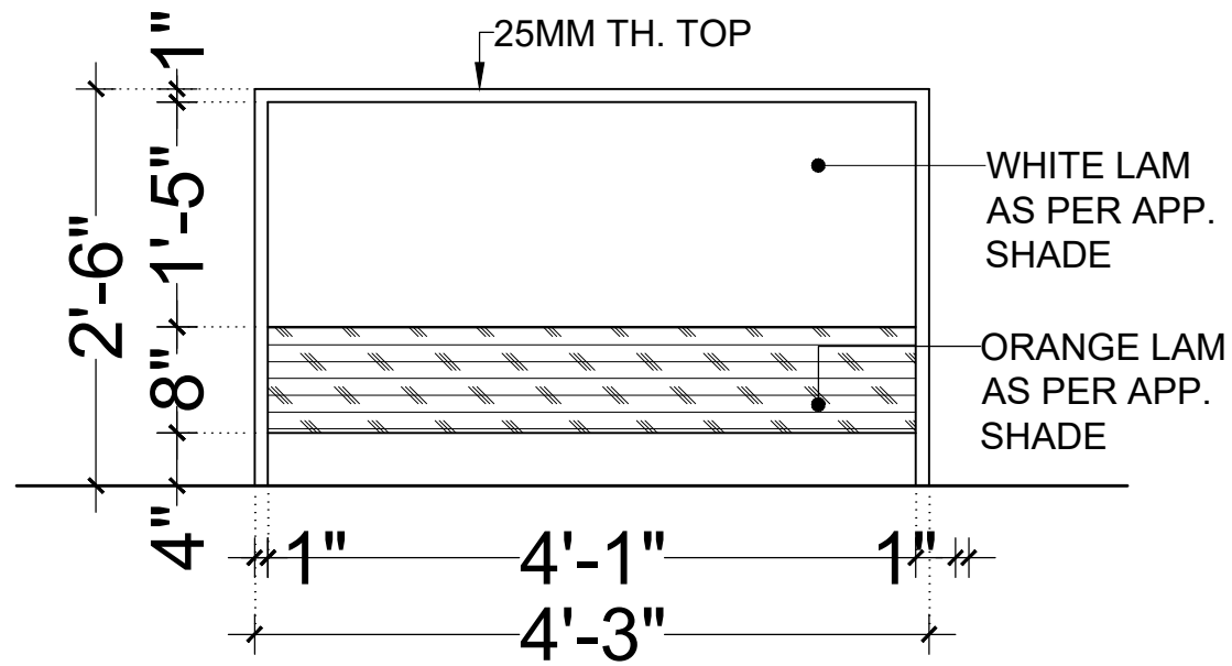
ELEVATION (FRONT) (OT2)
