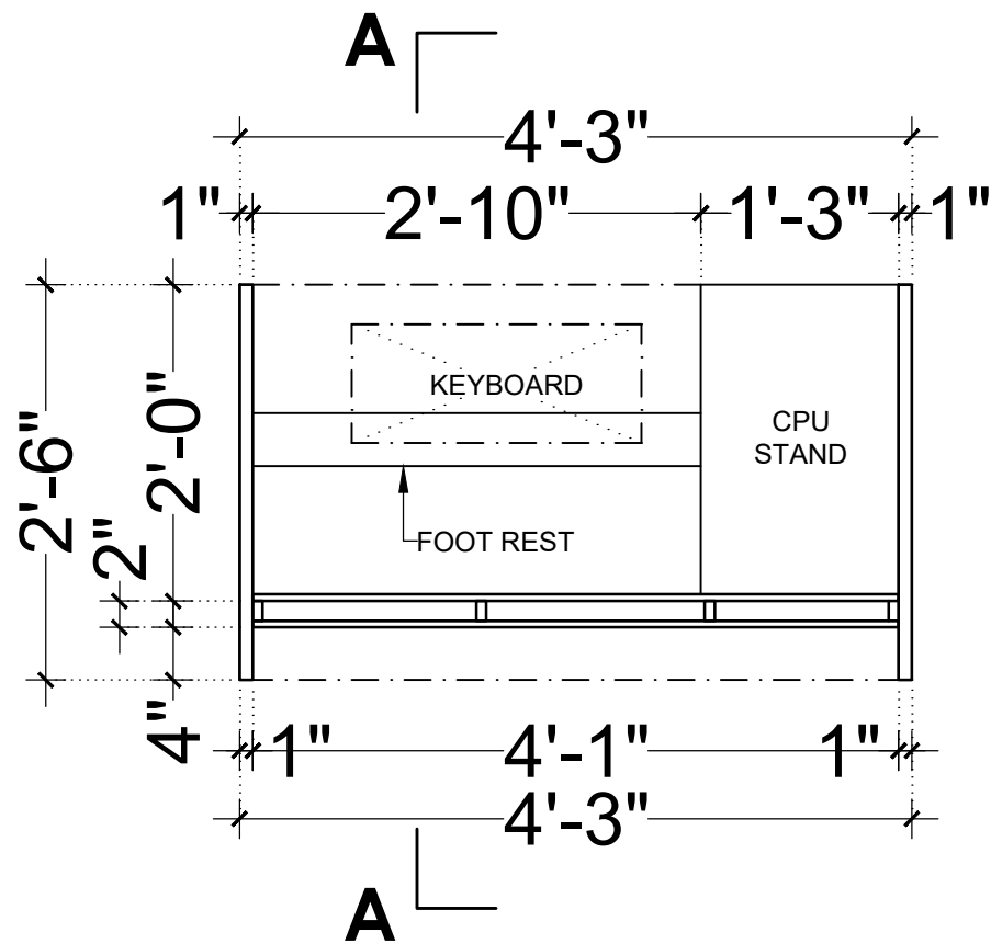
PLAN (LVL + 2'-0'') (OT1)
