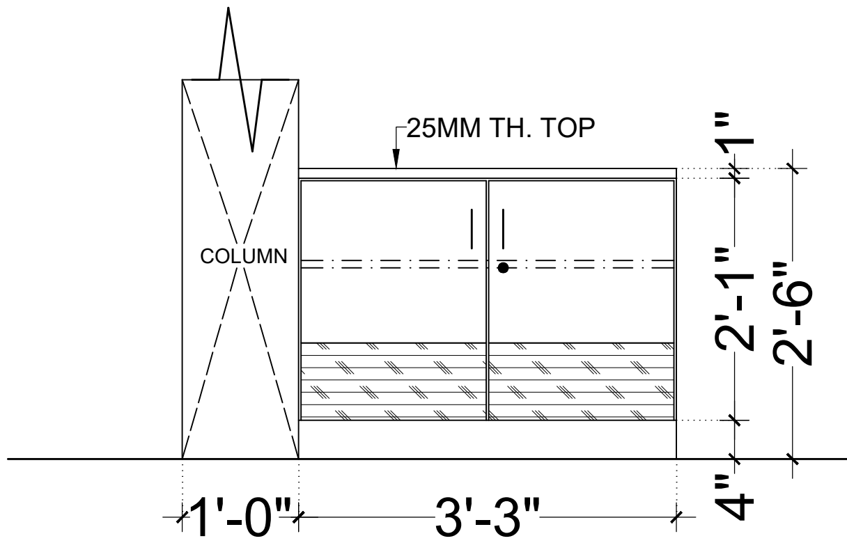
ELEVATION (FRONT) (SC2)
