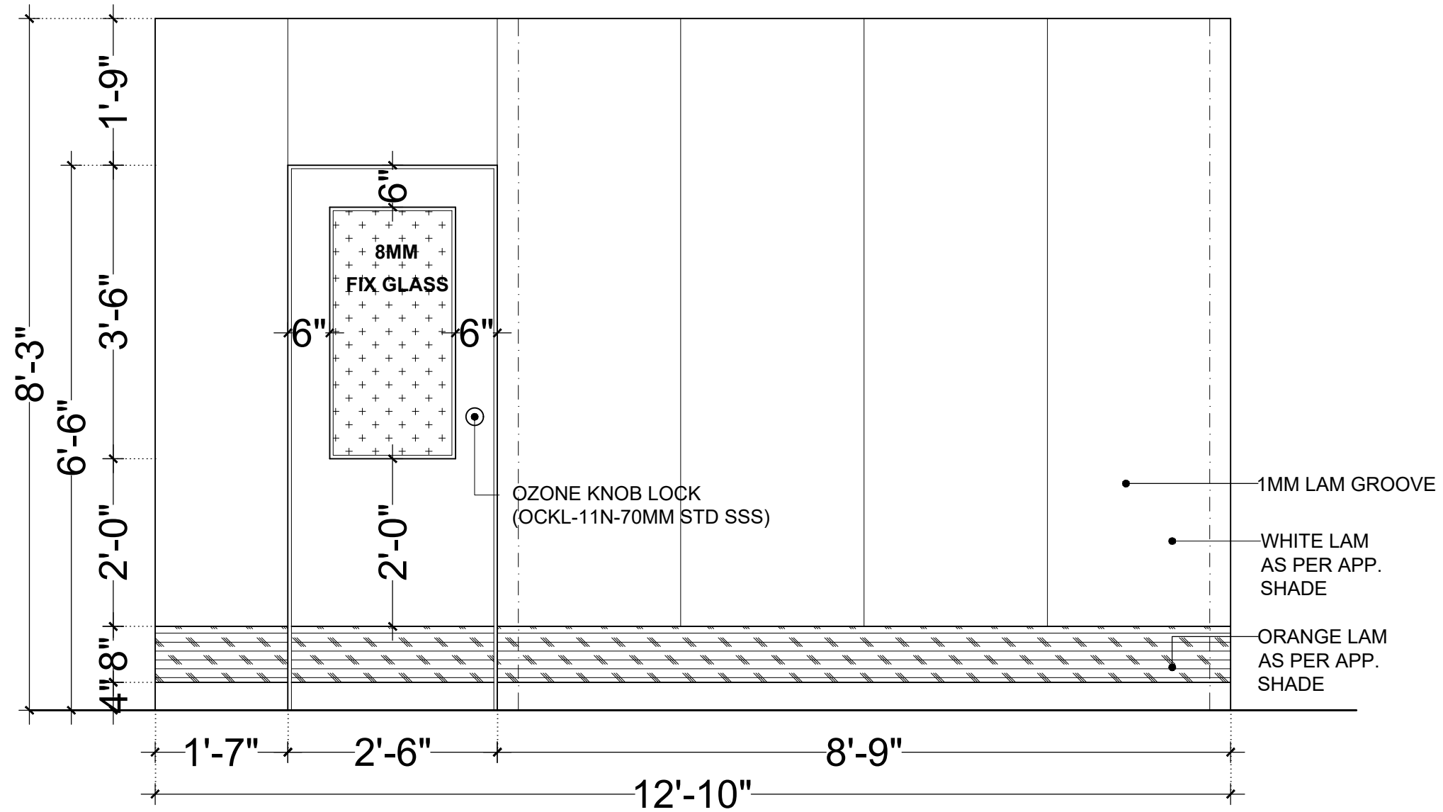
ELEVATION (PT5)
