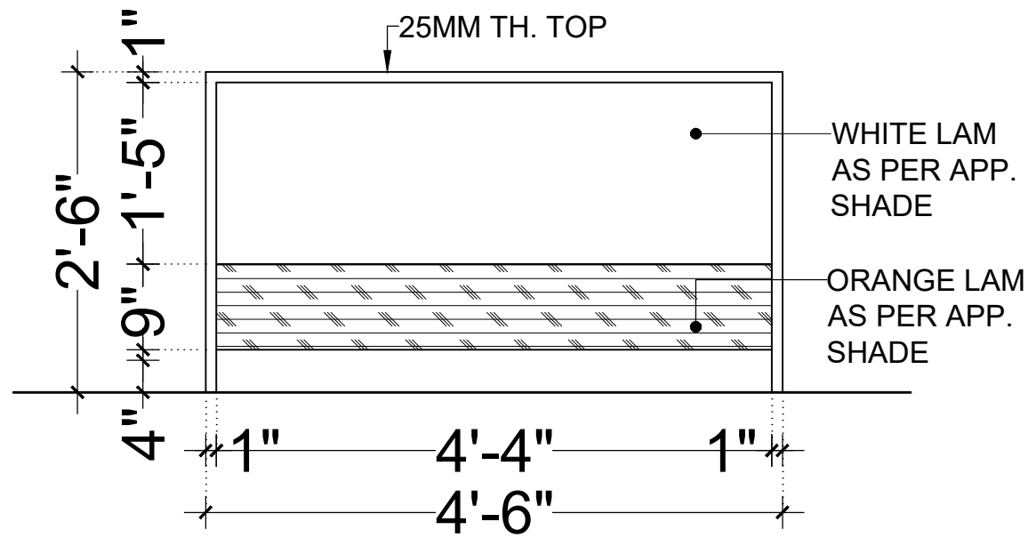
ELEVATION (FRONT) (OT4)
