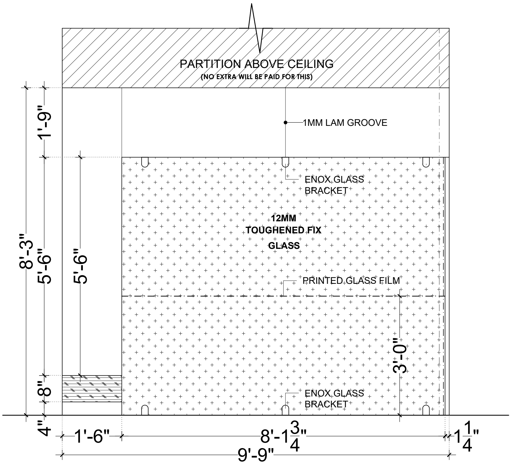
ELEVATION (PT1)
