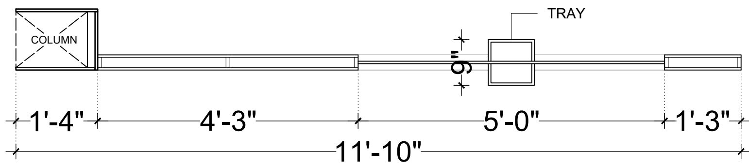
PLAN (PT3)
