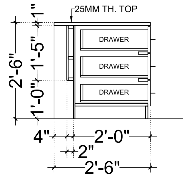
SECTION AA (MT1)
