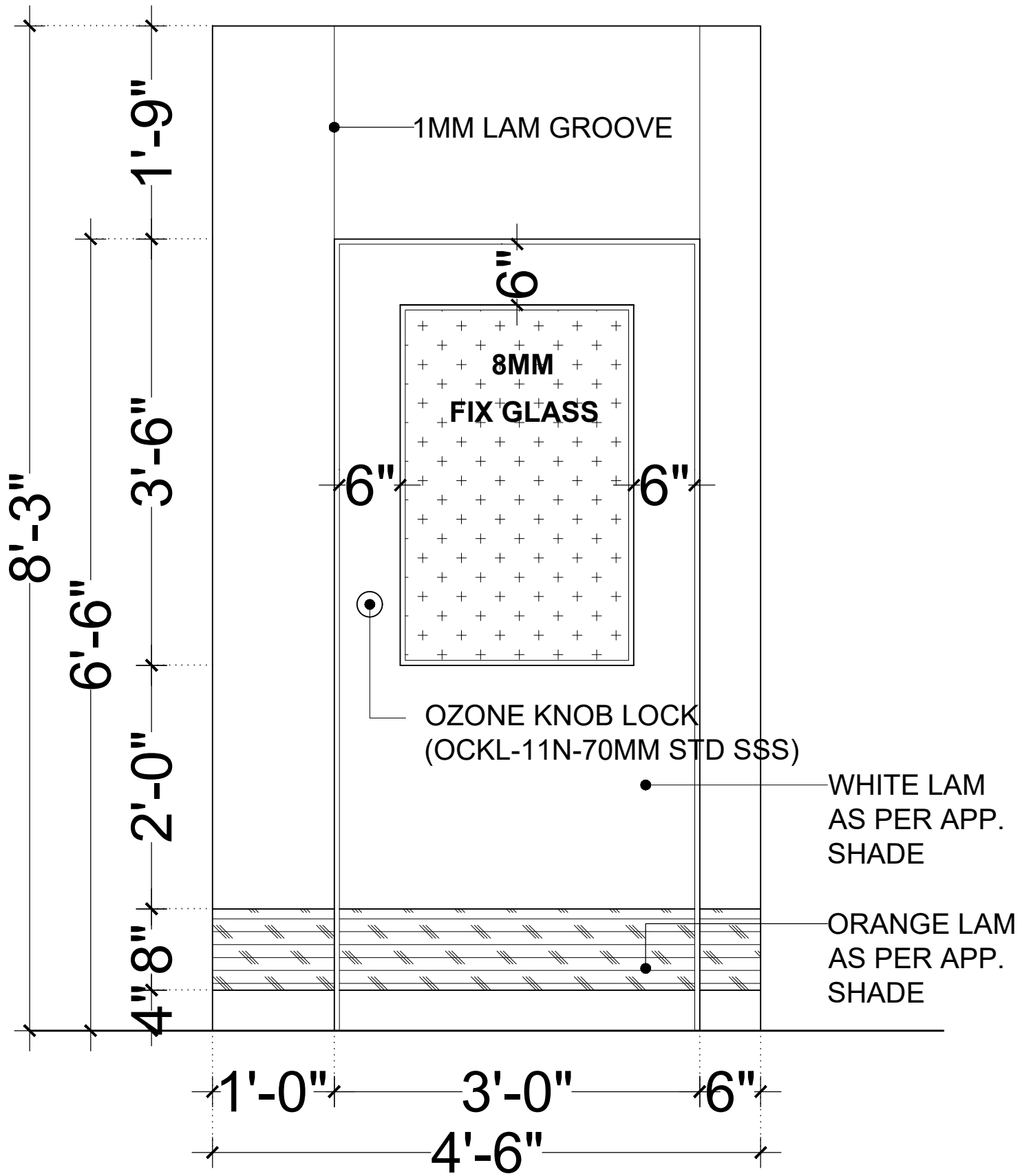
ELEVATION (PT10)
