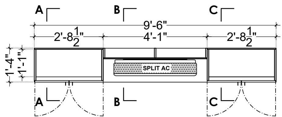
PLAN (CB3) (LVL + 7'-0")
