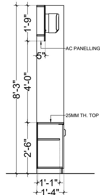
SECTION BB (CB4)
