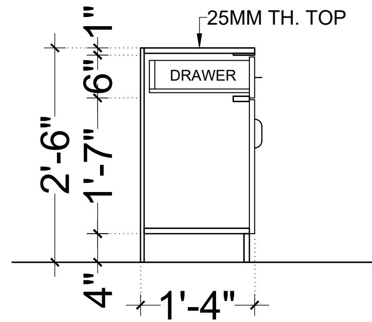
SECTION AA (SC1)
