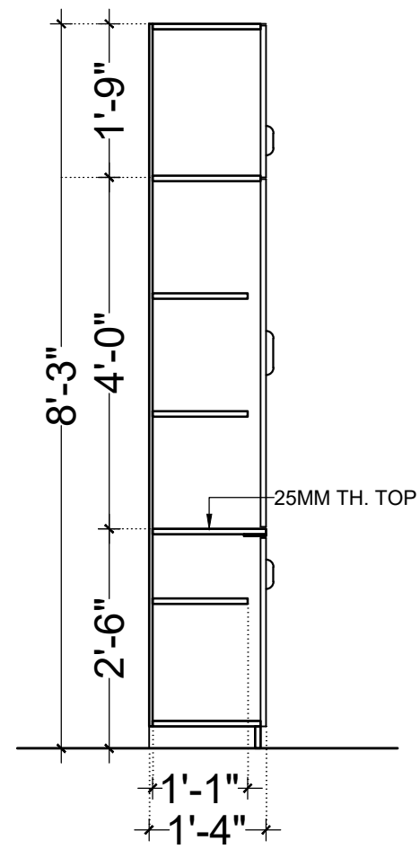
SECTION AA (CB5)
