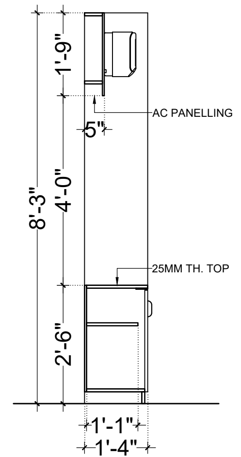
SECTION BB (CB1)
