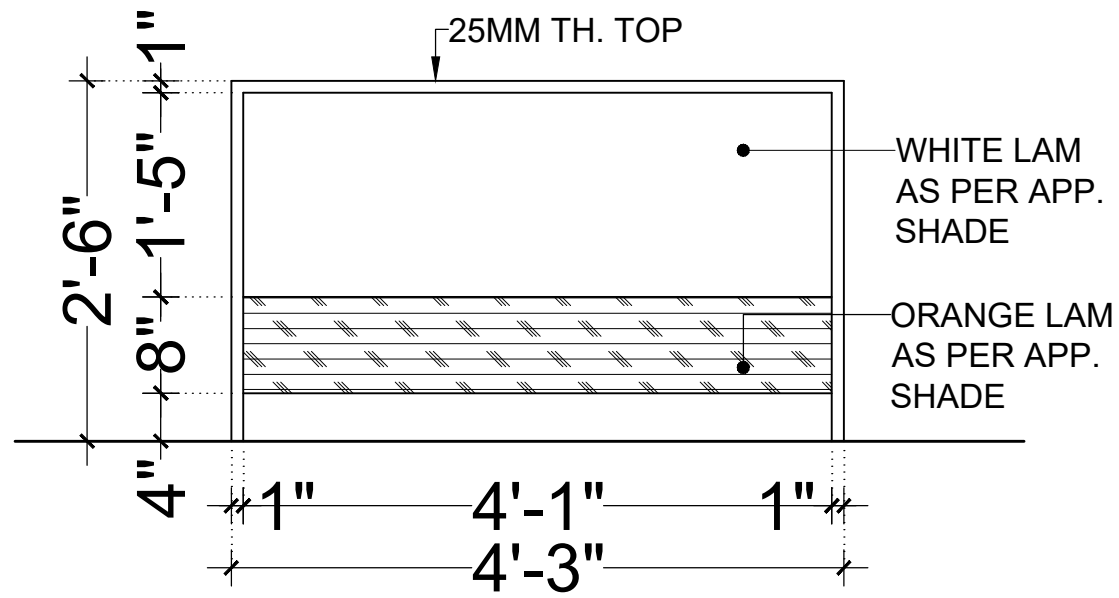
ELEVATION (FRONT) (OT1)
