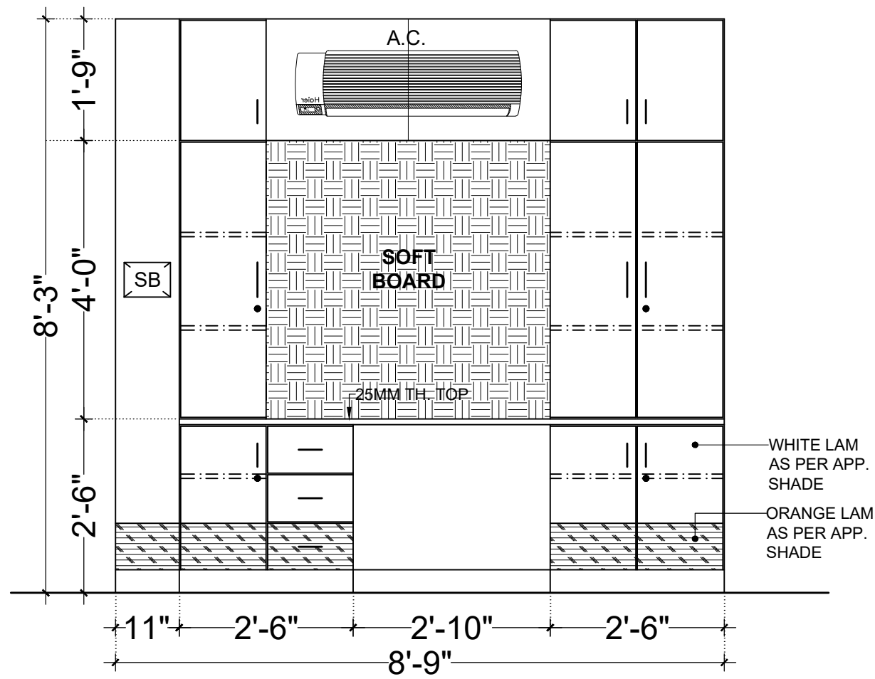
ELEVATION (CB5)
