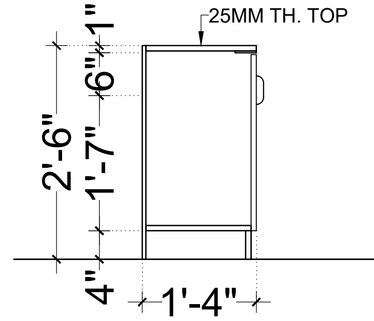
SECTION AA (SC2)
