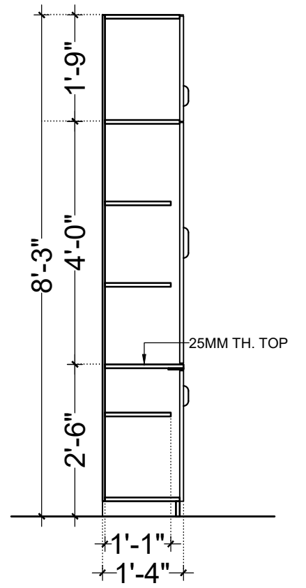
SECTION AA (CB2)
