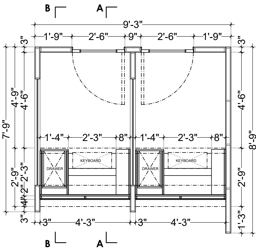
PLAN (CT1-1) (LVL + 2'-0'')
