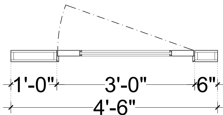
PLAN (PT10)
