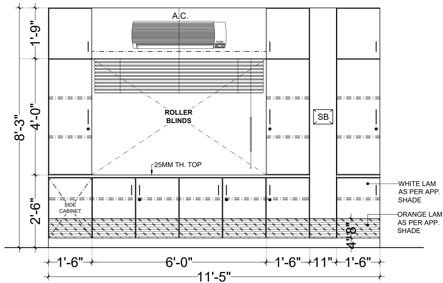
ELEVATION (CB1)
