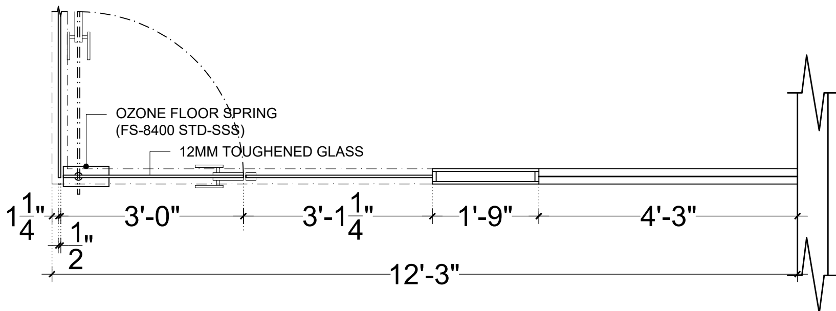
PLAN (PT2)
