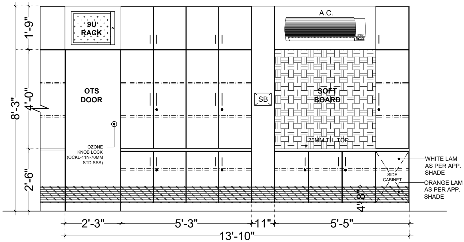
ELEVATION (CB2)
