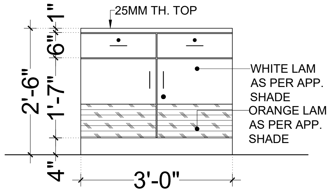
ELEVATION (FRONT) (SC1)
