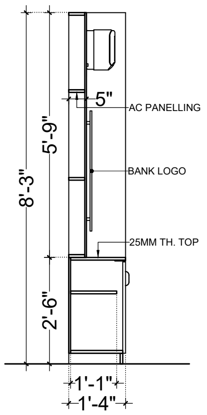
SECTION BB (CB3)
