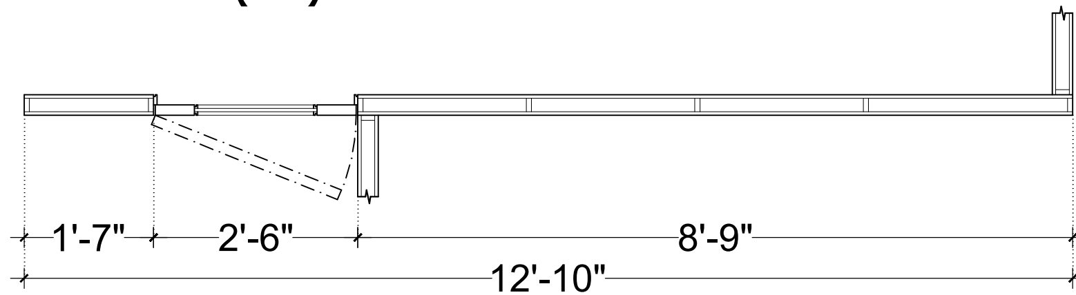
ELEVATION (PT5)
