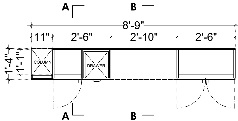
PLAN (CB5) (LVL + 2'-0")
