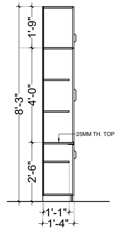
SECTION AA (CB4)
