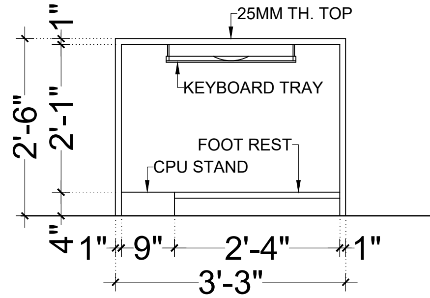
ELEVATION (INSIDE) (OT5)
