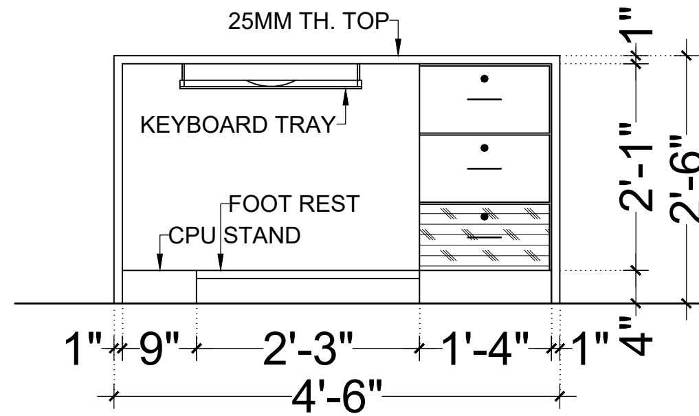
ELEVATION (INSIDE) (OT3)
