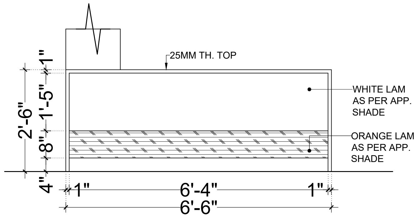
ELEVATION (FRONT) (MT1)
