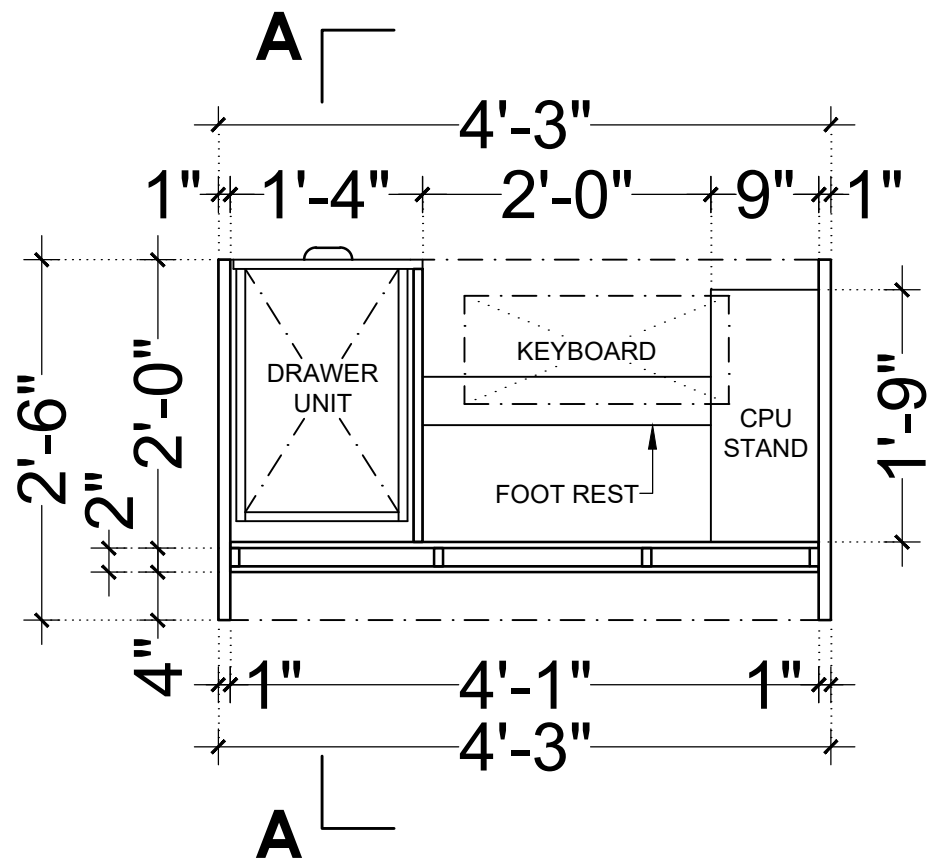
PLAN (LVL + 2'-0") (OT2)
