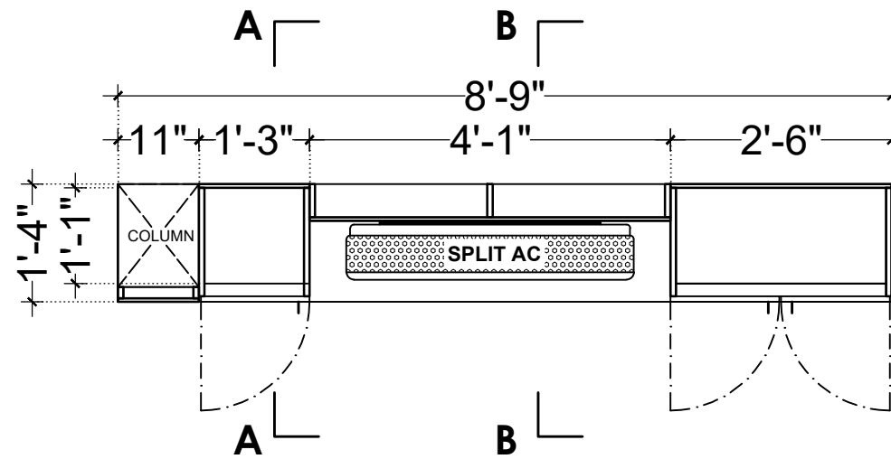
PLAN (CB5) (LVL + 7'-0")
