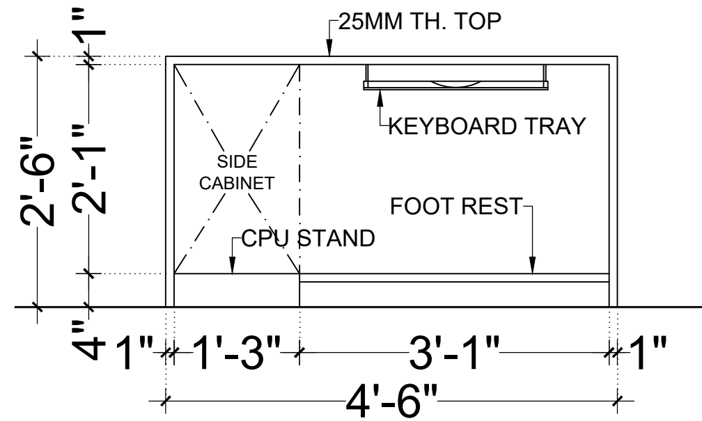
ELEVATION (INSIDE) (OT4)
