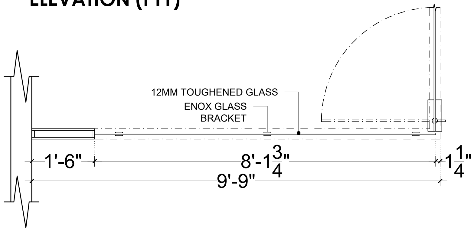
PLAN (PT1)
