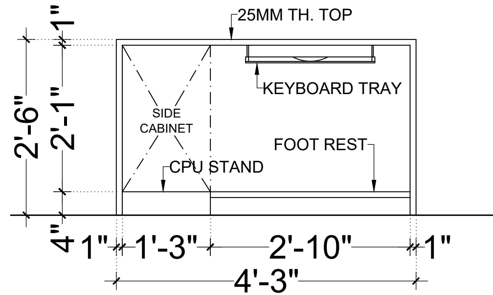
ELEVATION (INSIDE) (OT1)
