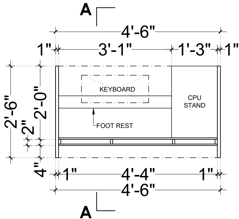
PLAN (LVL + 2'-0'') (OT4)
