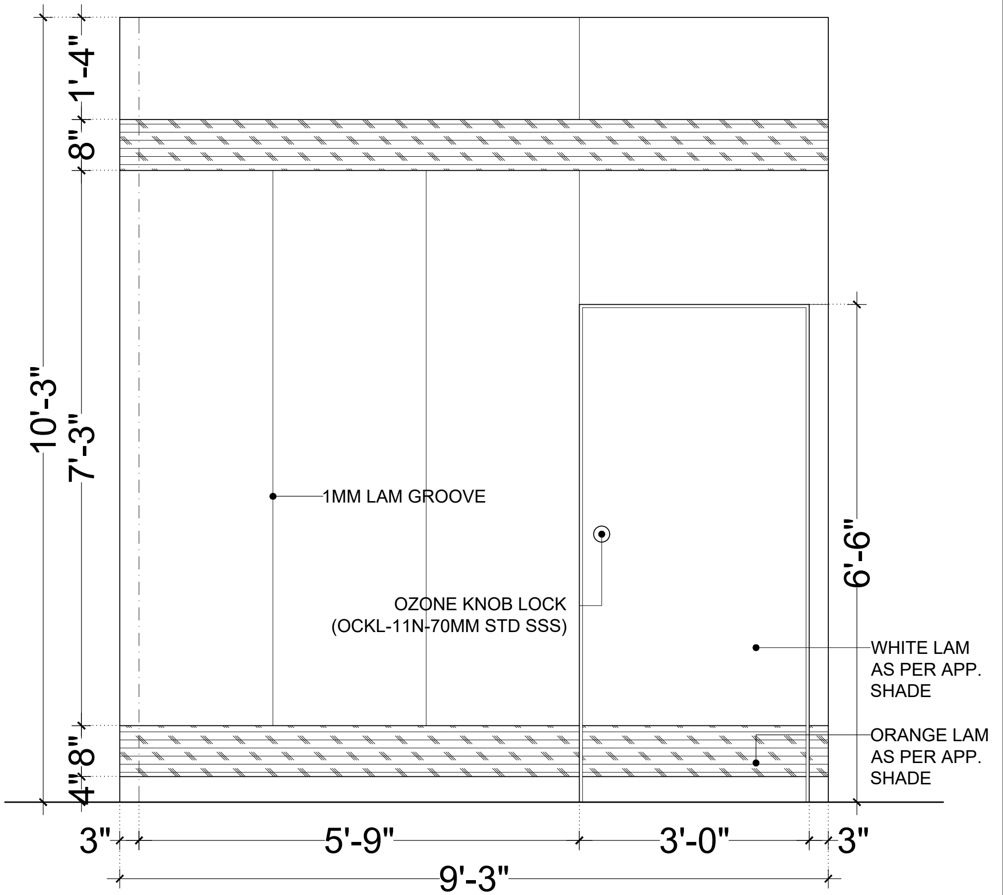
ELEVATION (PT8)
