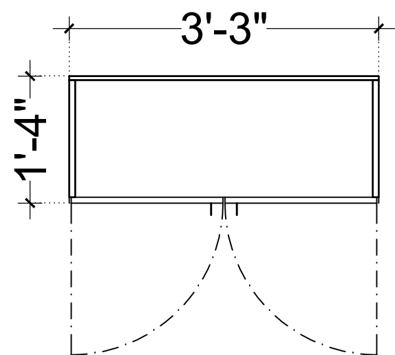
PLAN (CB6) (LVL + 5'-0")
