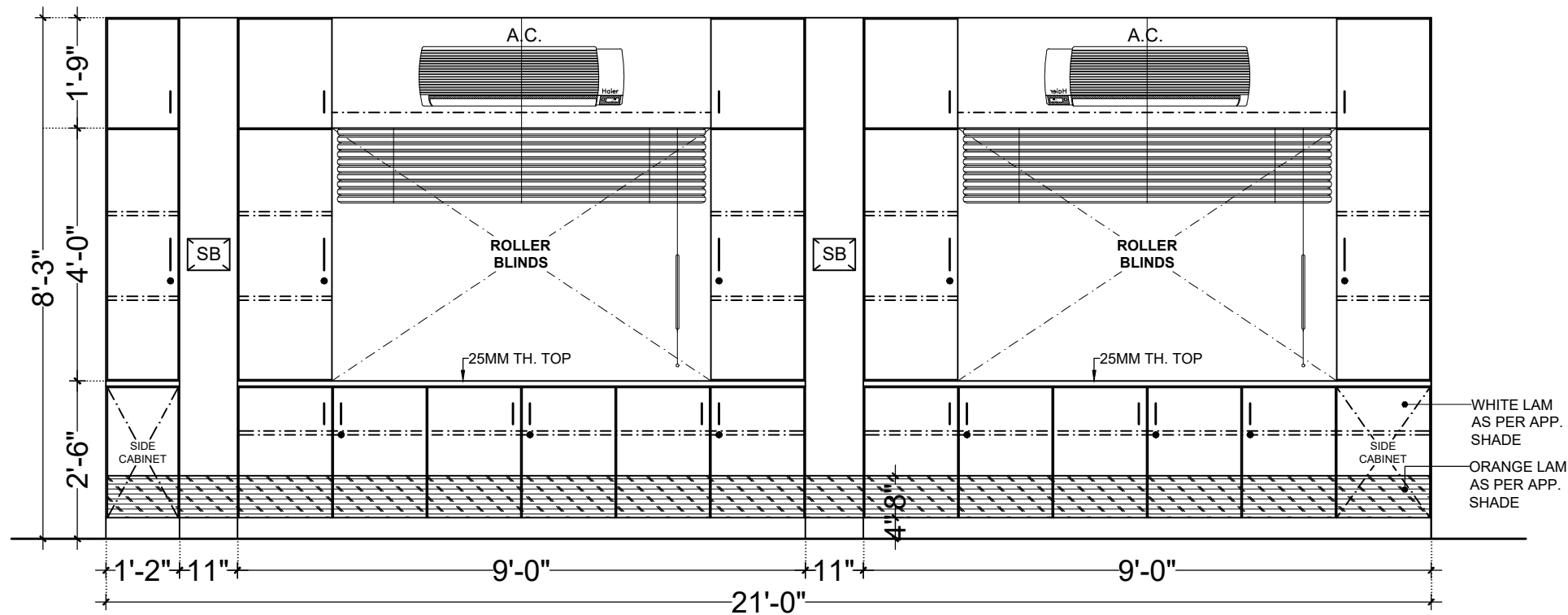
ELEVATION (CB4)
