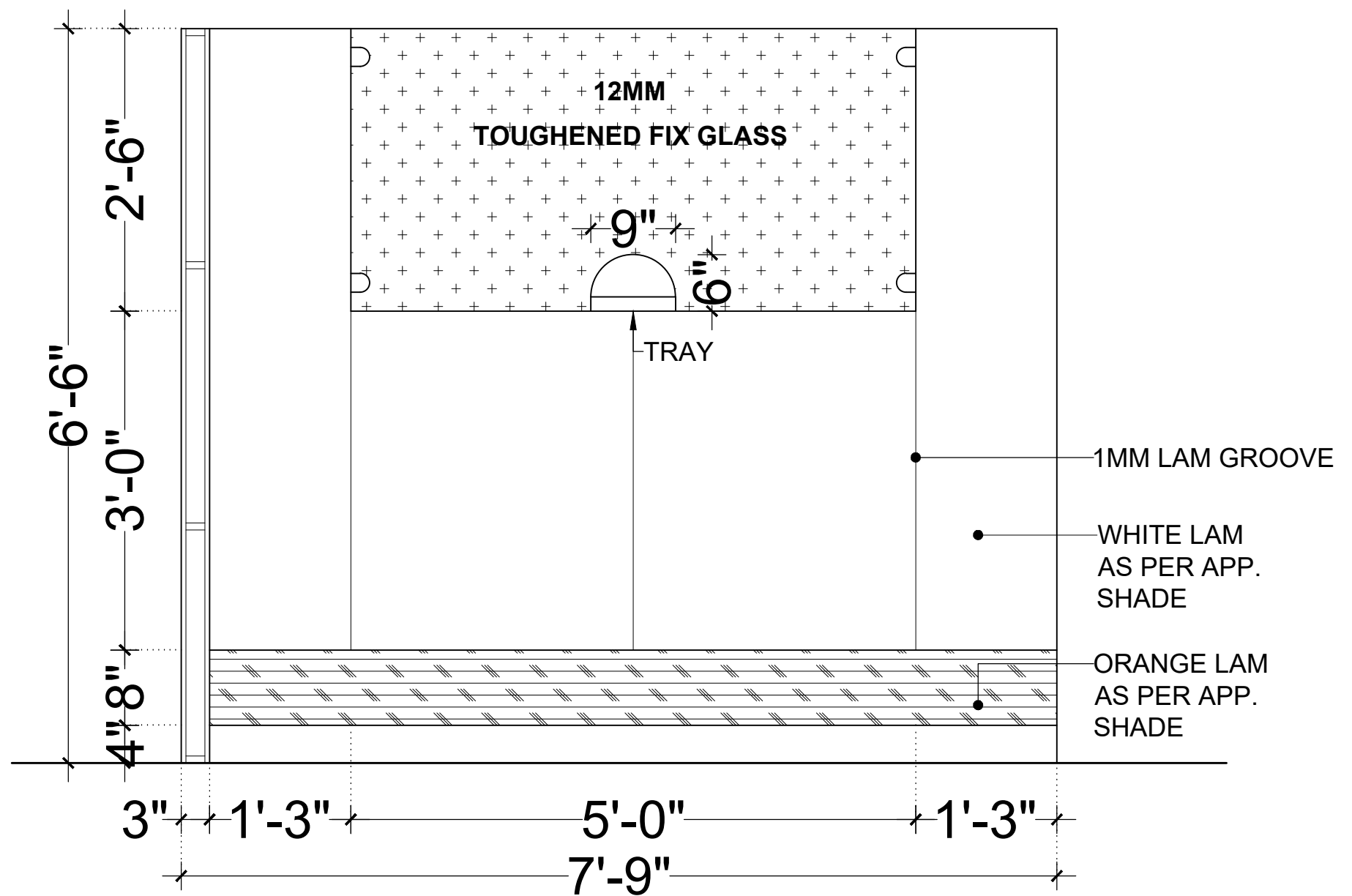
ELEVATION (PT4)
