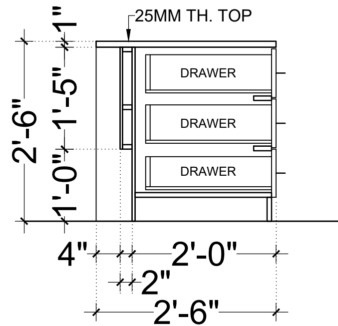
SECTION AA (OT2)
