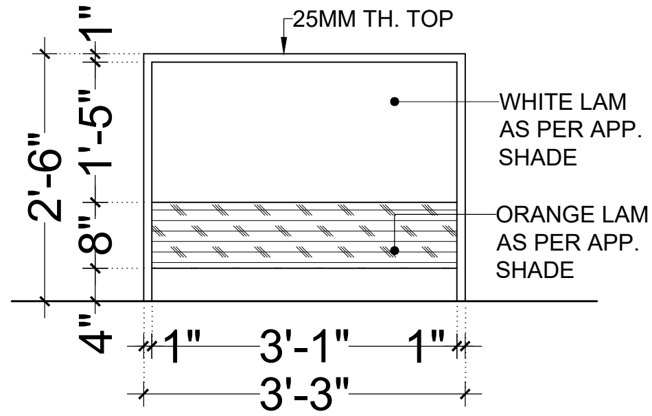
ELEVATION (FRONT) (OT5)
