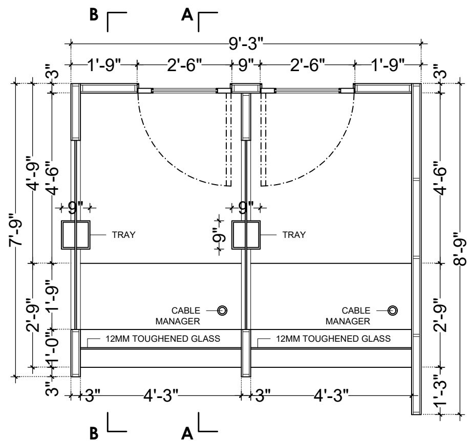
PLAN (CT1-1) (LVL + 5'-0'')
