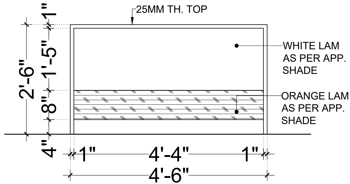
ELEVATION (FRONT) (OT3)
