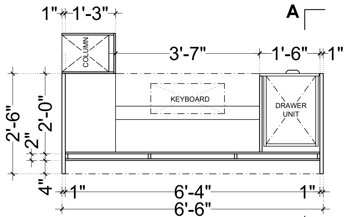
PLAN (LVL + 2'-0") (MT1)
