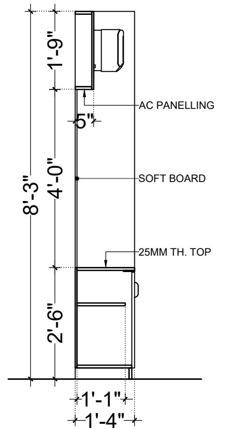
SECTION BB (CB2)
