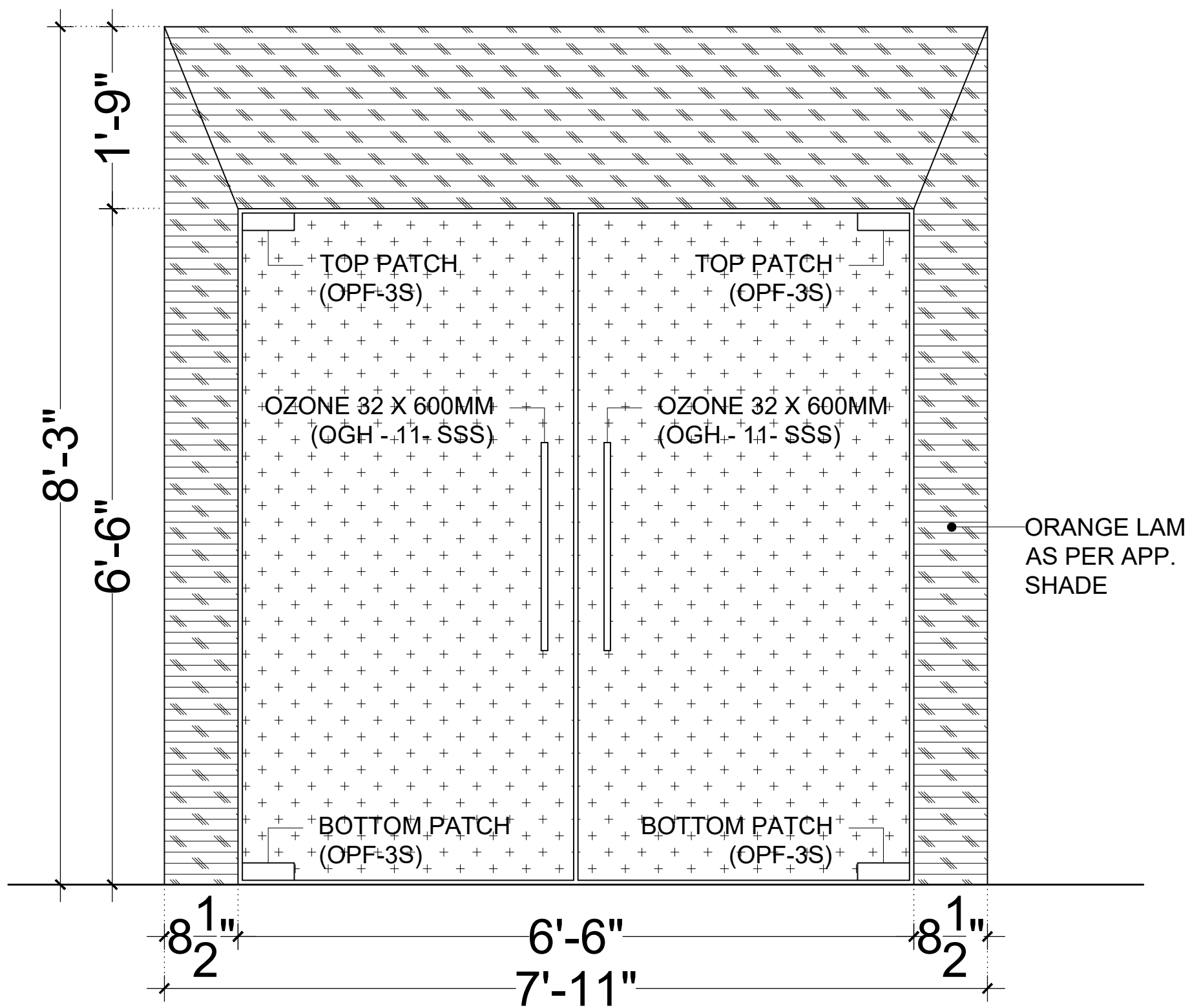
ELEVATION (PT11)
