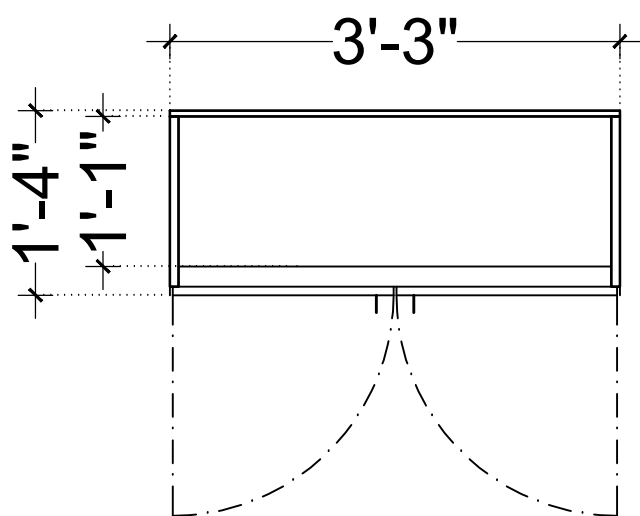
PLAN (CB6) (LVL + 2'-0")
