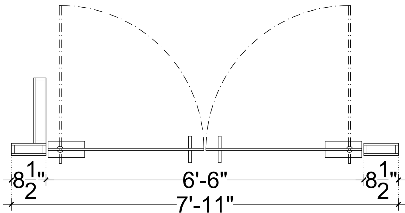
PLAN (PT11)
