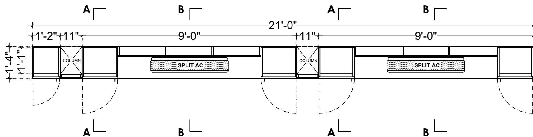
PLAN (CB4) (LVL + 7'-0")
