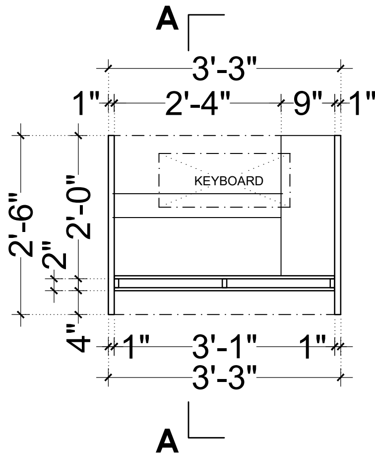
PLAN (LVL + 2'-0") (OT5)
