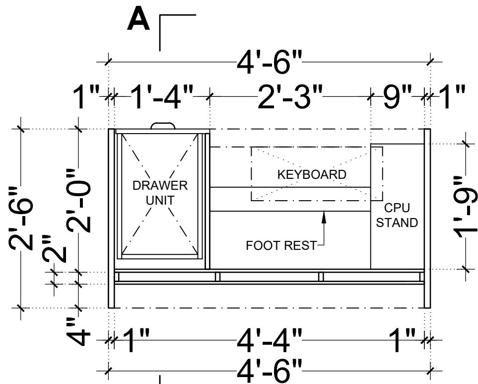
ELEVATION (FRONT) (OT3)
