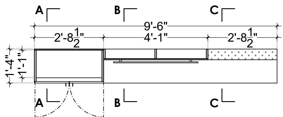
PLAN (CB3) (LVL + 5'-0")
