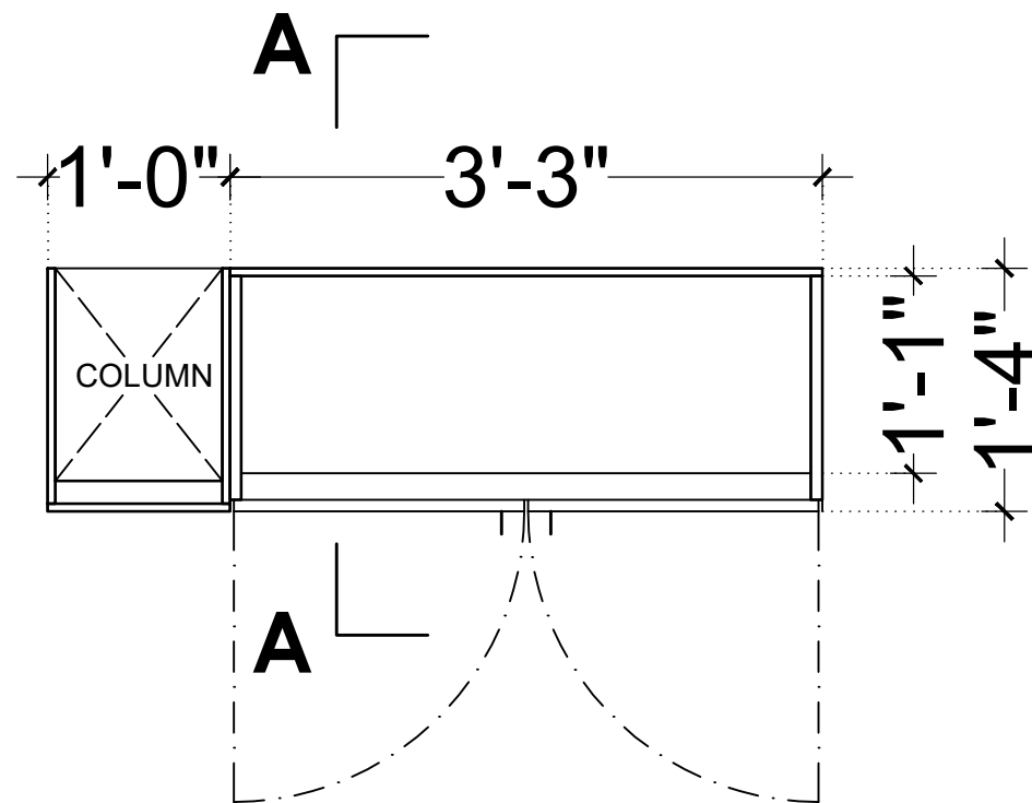
PLAN (LVL + 1'-6") (SC2)
