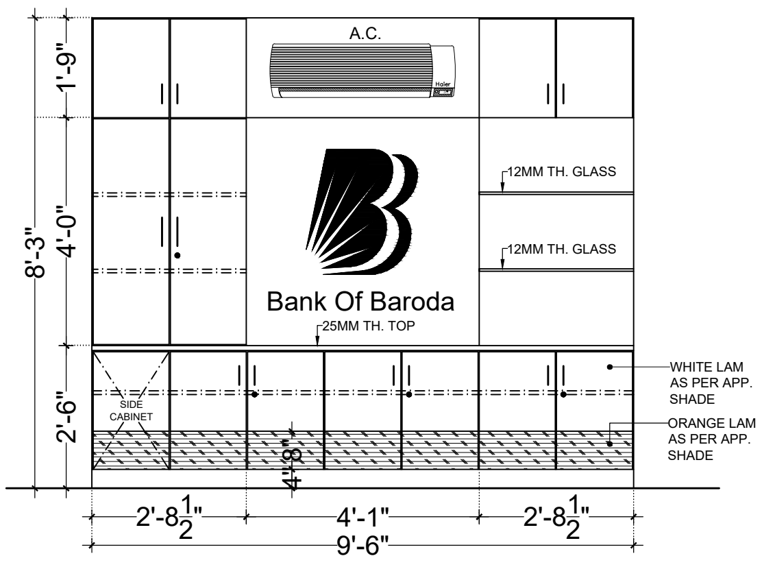
ELEVATION (CB3)
